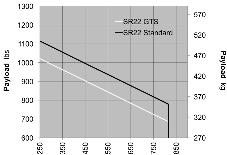
SR22 High Speed Cruise @ 8,000 Ft (180 KTAS)
