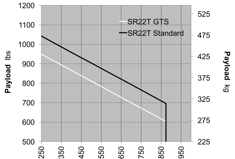
SR22T High Speed Cruise @ 18,000 Ft (198 KTAS)
