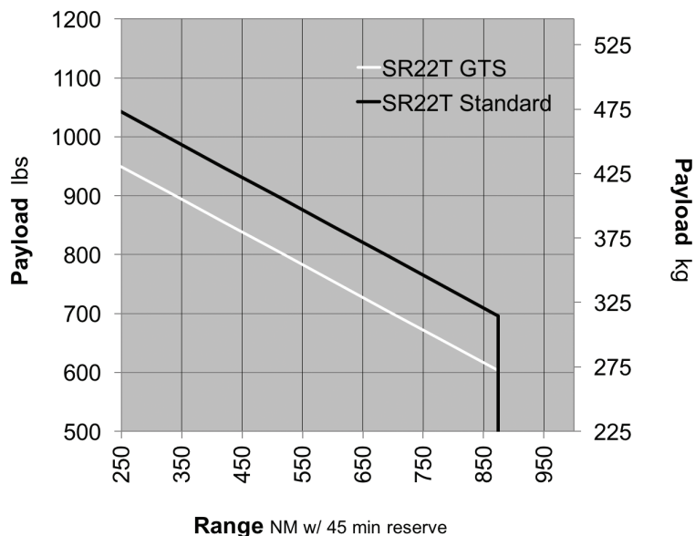
SR22T High Speed Cruise @ 18,000 Ft (198 KTAS)
