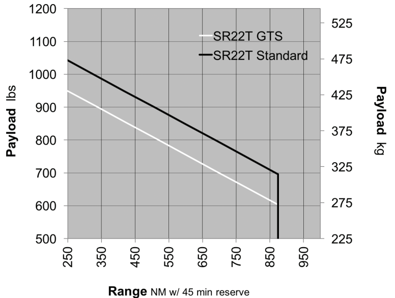
SR22T High Speed Cruise @ 18,000 Ft (198 KTAS)
