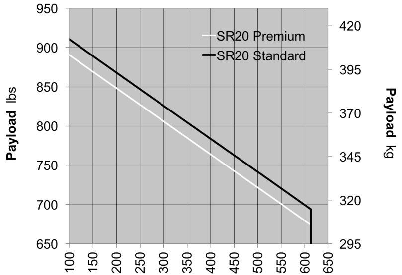
Range NM w/ 45 min reserve
