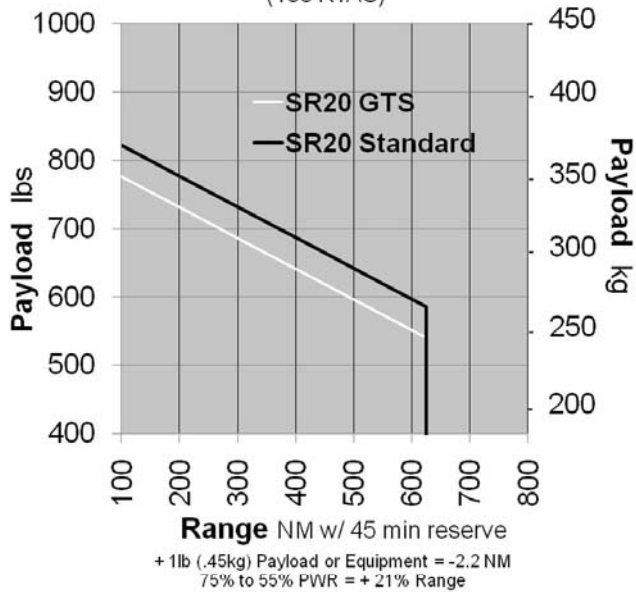
SR20 High Speed Cruise @ 8,000 Ft (155 KTAS)
