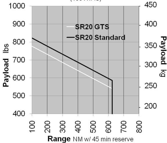
SR20 High Speed Cruise @ 8,000 Ft (155 KTAS)
